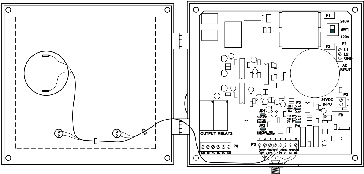
Figure 1 FluidWatch Configuration
